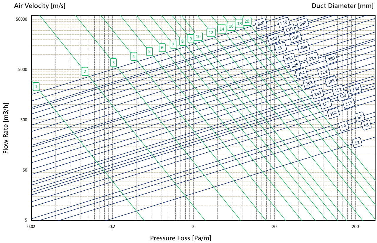
Pressure loss chart for COM-F
